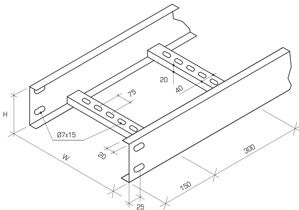
THANG THẲNG / STRAIGHT SECTION Mã đặt hàng/ Order code: SL-WxHxT
