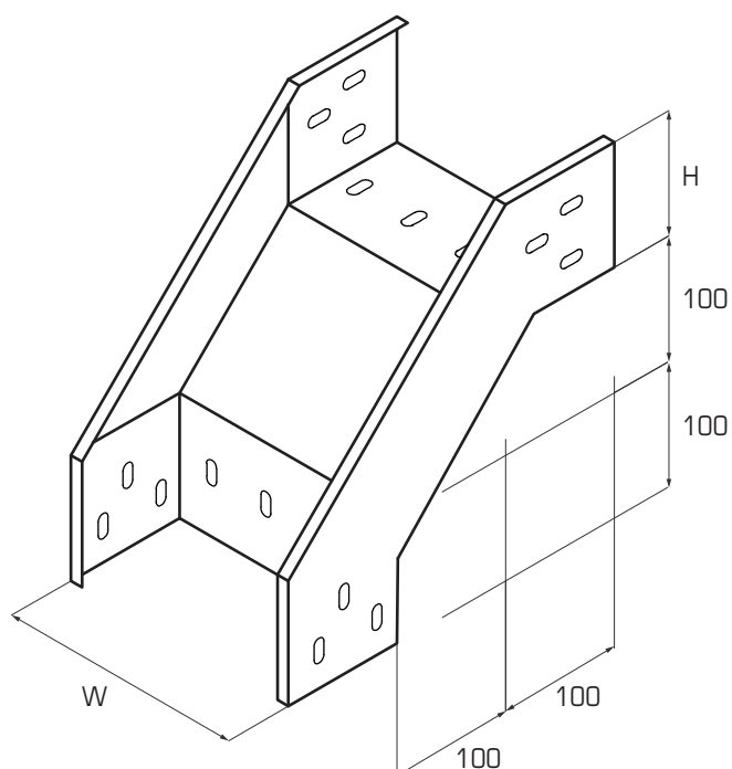
CO XUỐNG/ VERTICAL BEND (DOWN) Mã đặt hàng/ Order code: EBTH-WxHxT
